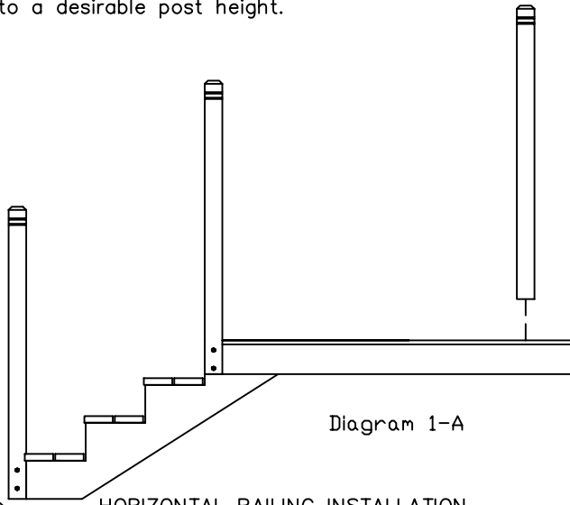
HORIZONTAL RAILING INSTALLATION
